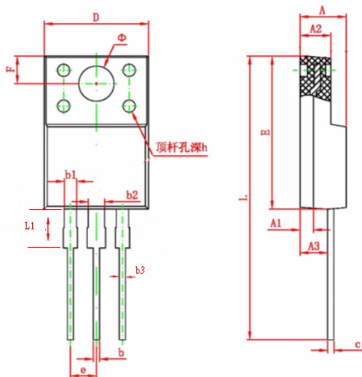
TO-220FP
