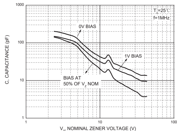
Fig. 5 Typical Capacitance
