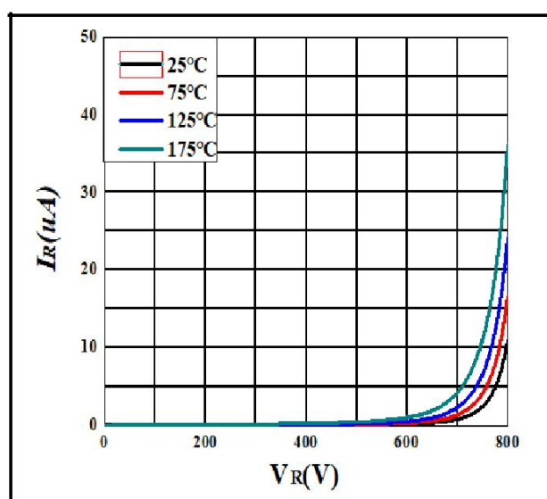
Figure 2. Reverse Characteristics
