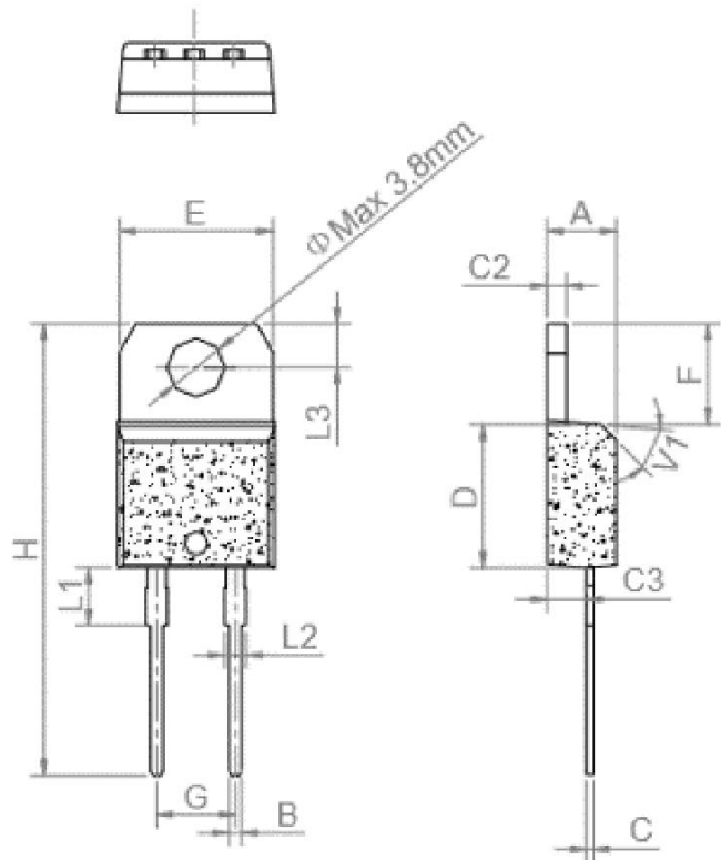
TO-220N-2L
