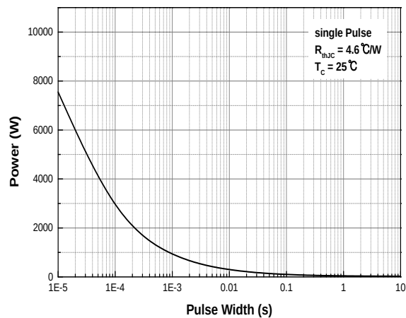
Fig.12 Single Pulse Maximum Power Dissipation- MDF5N50F (TO-220F)
