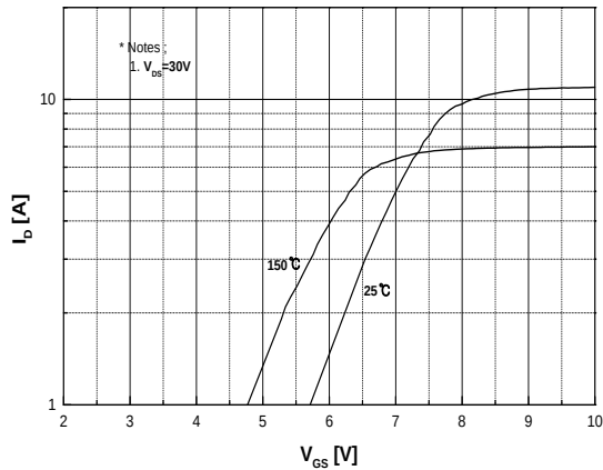
Fig.5 Transfer Characteristics
