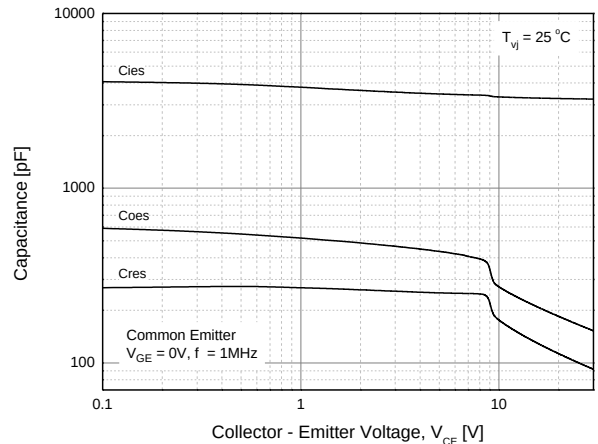
Fig. 6 IGBT Capacitance Characteristics
