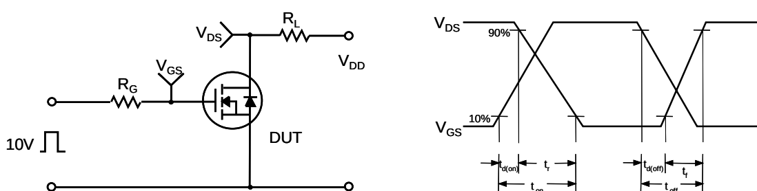
Resistive Switching Test Circuit &amp; Waveforms
