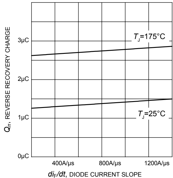
Figure 24. Typical reverse recovery charge as a function of diode current slope ( V_R=600\text{V} , I_F=15\text{A} , Dynamic test circuit in Figure E)
