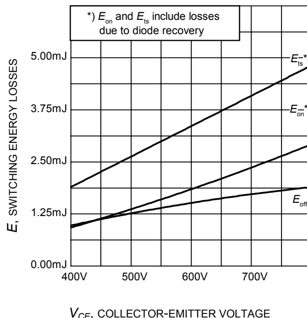
Figure 16. Typical switching energy losses as a function of collector emitter voltage (inductive load, T_J=175^\circ\text{C} , V_{GE}=0/15\text{V} , I_C=15\text{A} , R_G=41.8\Omega , Dynamic test circuit in Figure E)
