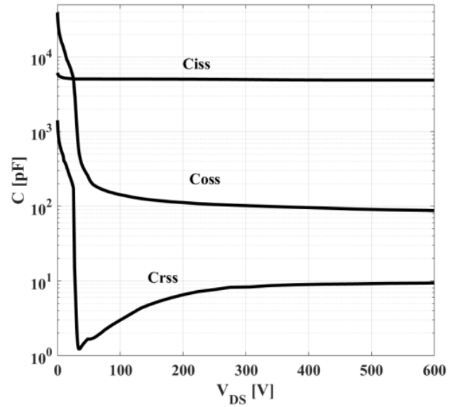
Figure 16: Typ. Capacitances
