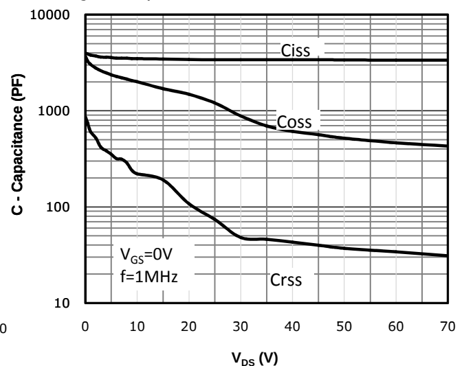
Fig 6: Capacitance Characteristics
