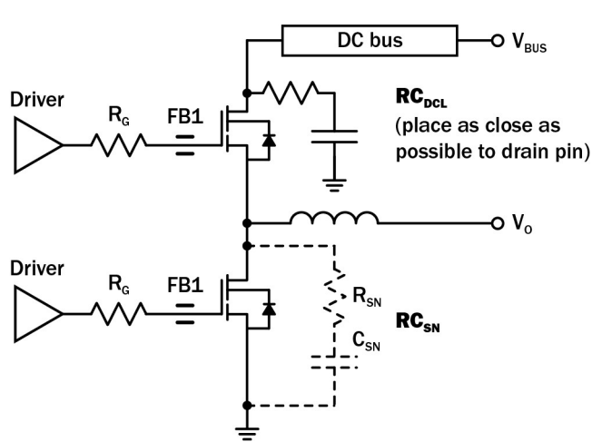
Simplified Half-bridge Schematic
