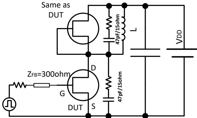
Figure 1. Switching Time Test Circuit (see circuit implementation on page 3 for methods to ensure clean switching)
