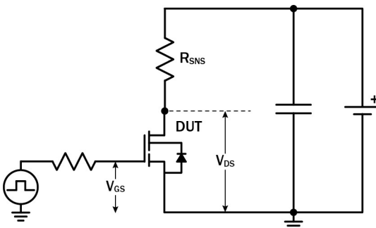
Figure 5. Dynamic R_{DS(on)eff} Test Circuit
